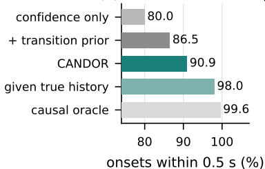
(a) the selection ceiling
