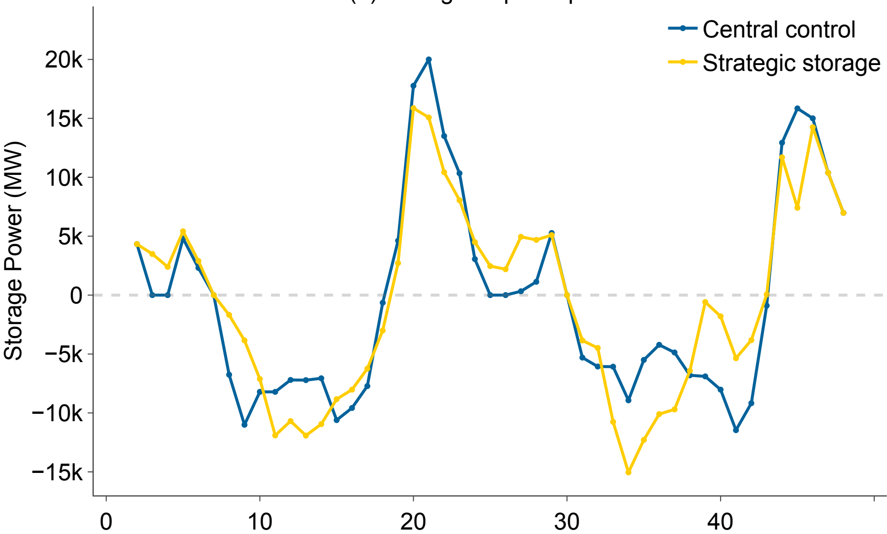
(a) Storage dispatch profile
