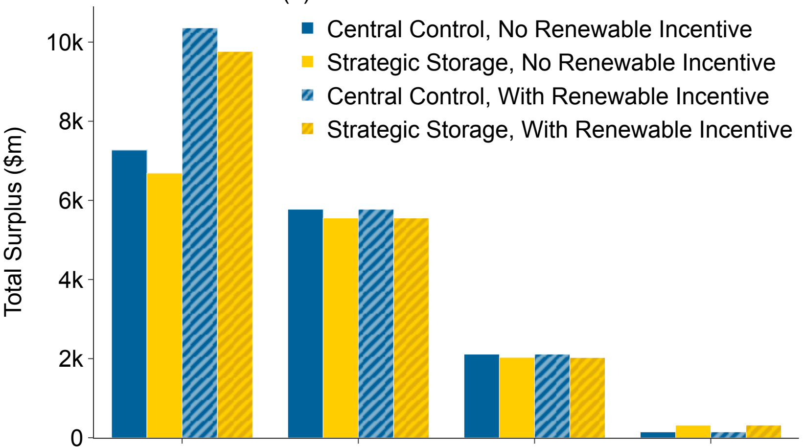
(a) 40% VRE Generation Share
