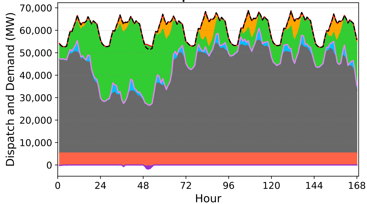
SpotMLT
