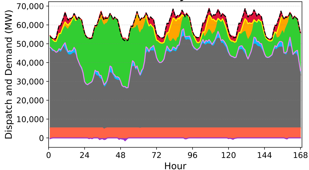
SpotMLT
