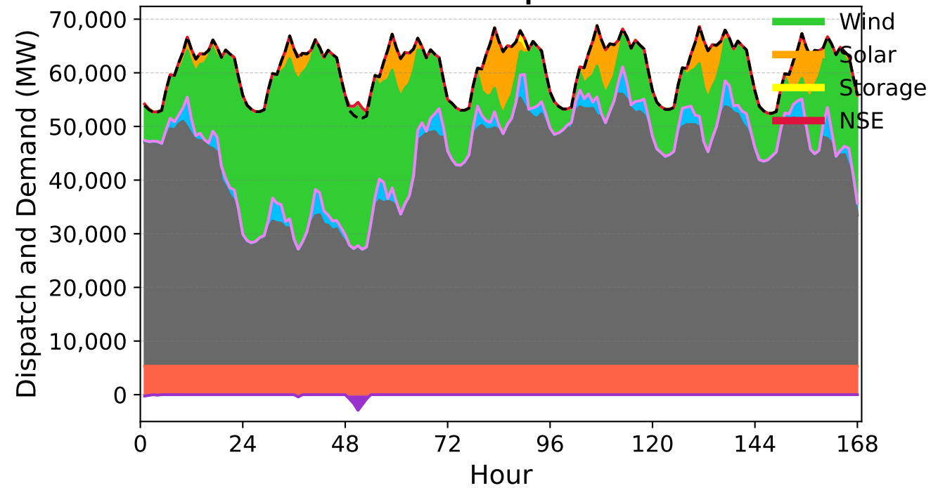
FlexibleSpotMLT
