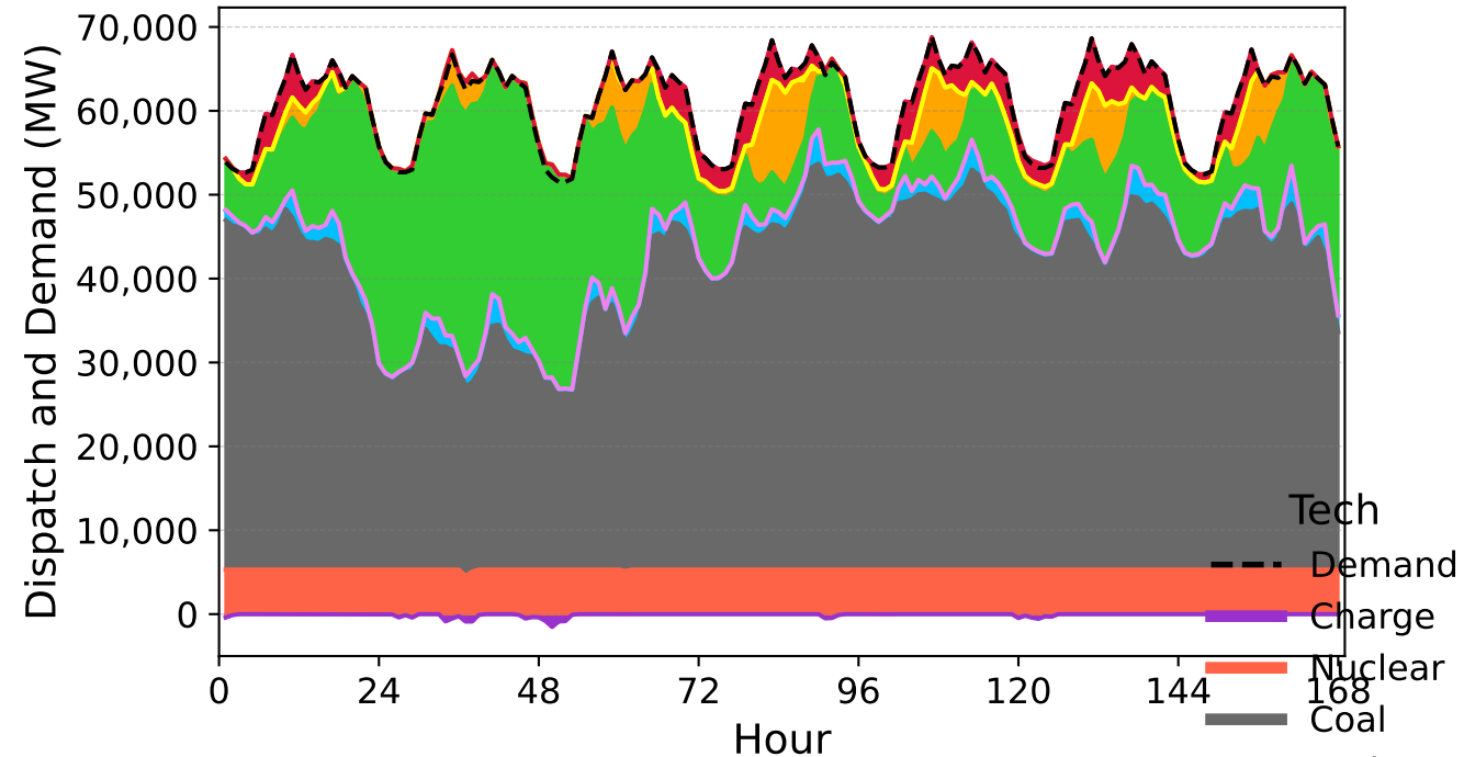
FlexibleSpotMLT
