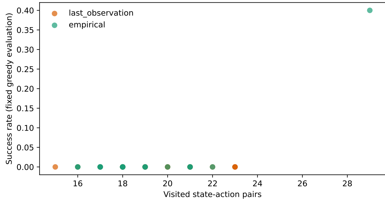
Stochasticity exposes the model-quality boundary
