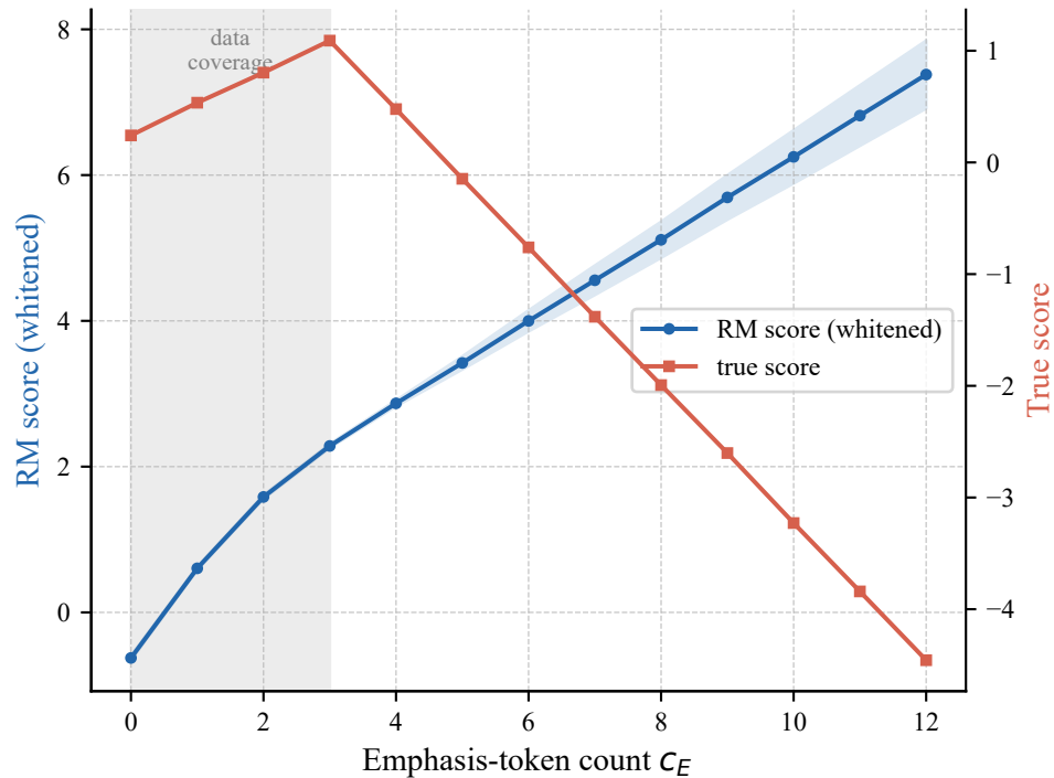
In-support agreement, out-of-support divergence
