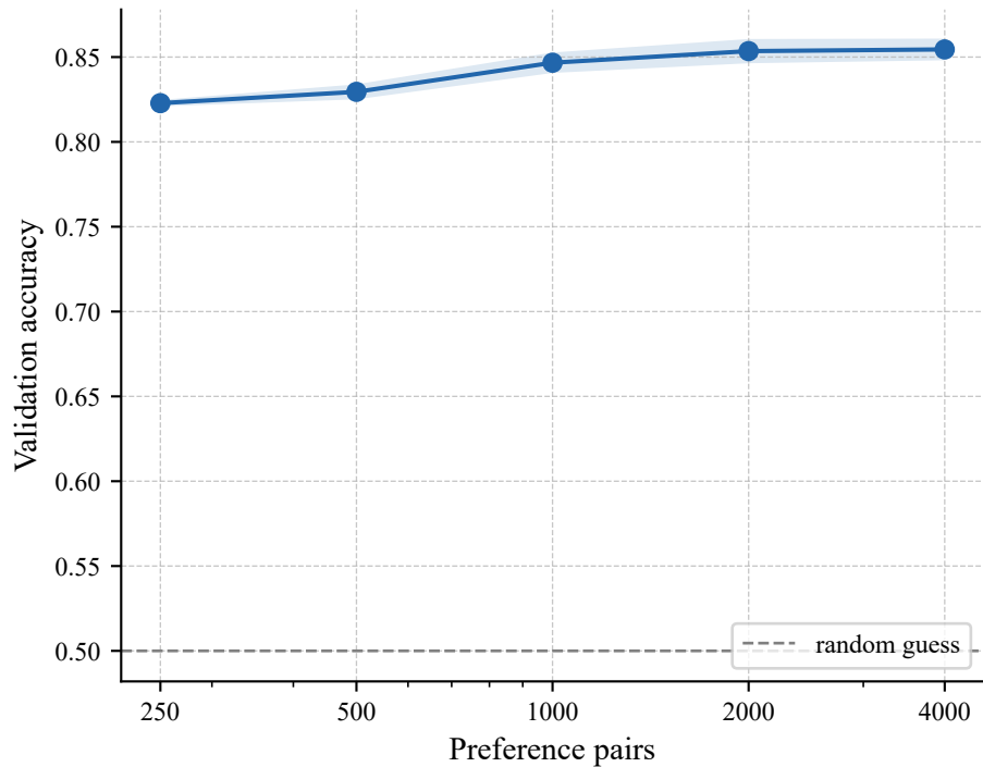
Reward model accuracy vs data
