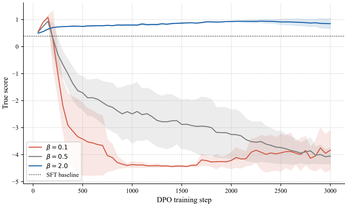
Fig 3. The DPO anchor loosens with training (3 seeds, mean \pm std)
