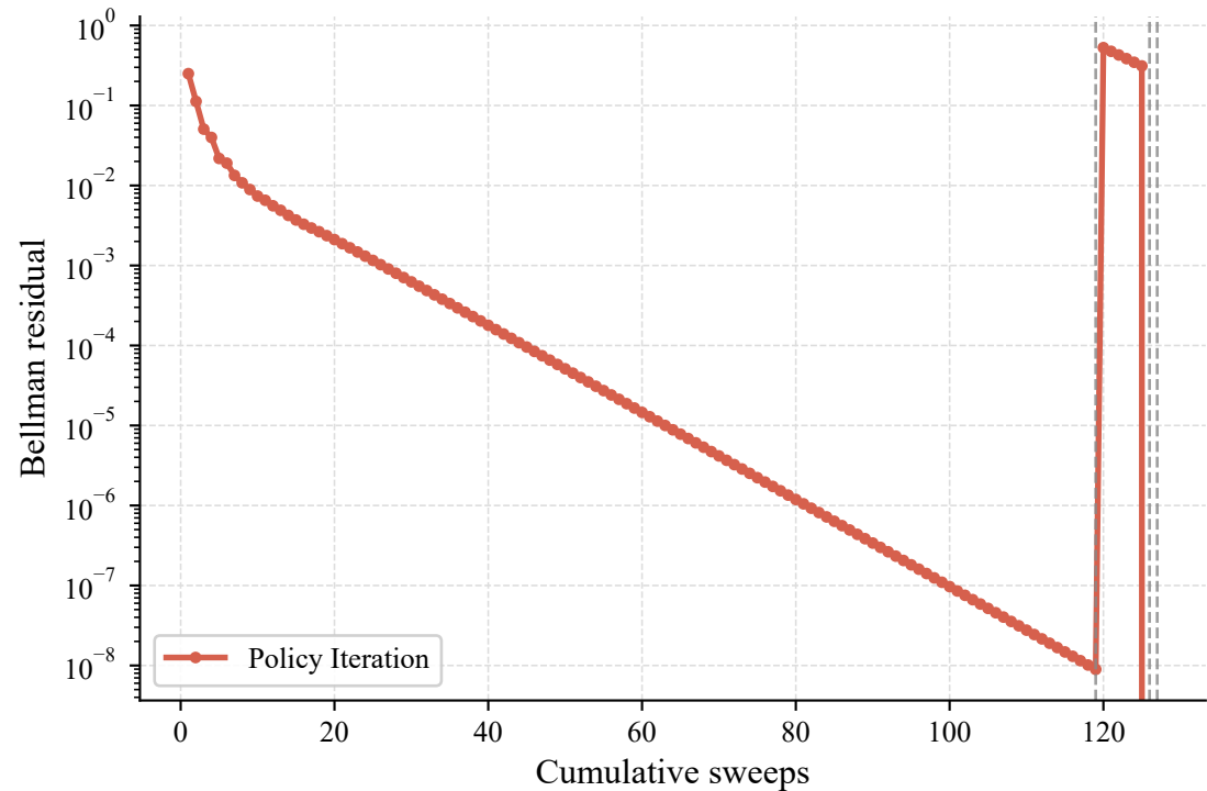
Policy Iteration: Residual per Sweep (3 iterations, dashed = policy improvement)
