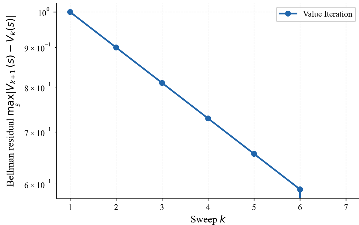
Value Iteration: Residual Decay
