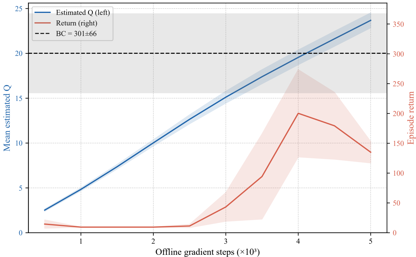
Fig 1. Naive offline DQN: Q diverges from return (CartPole-v1, medium)
