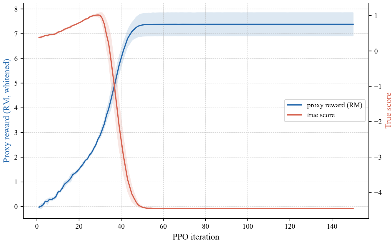
Fig 2. Reward hacking under \beta = 0 (3 seeds, mean \pm std)
