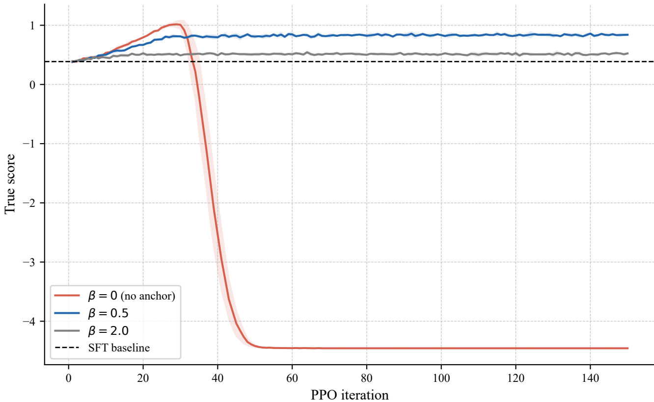
Fig 3. KL anchoring (3 seeds, mean \pm std)
