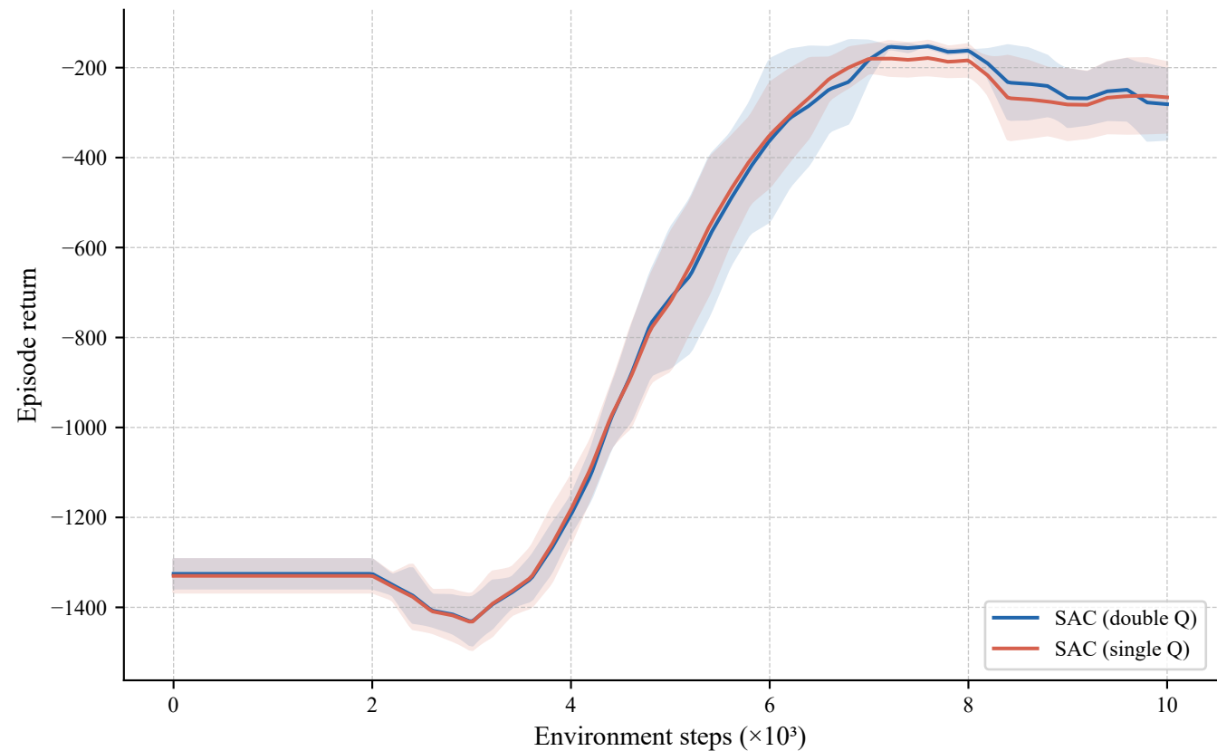
Fig 2. Double Q vs single Q on Pendulum-v1
