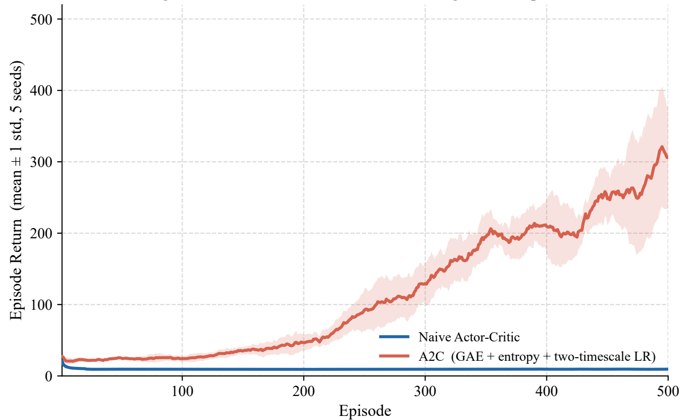
Fig 2. A2C vs. Naive Actor-Critic: Convergence Comparison
