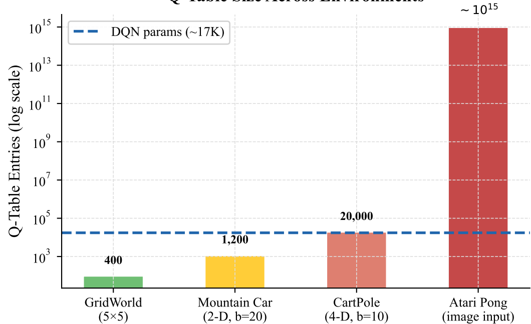
Q-Table Size Across Environments
