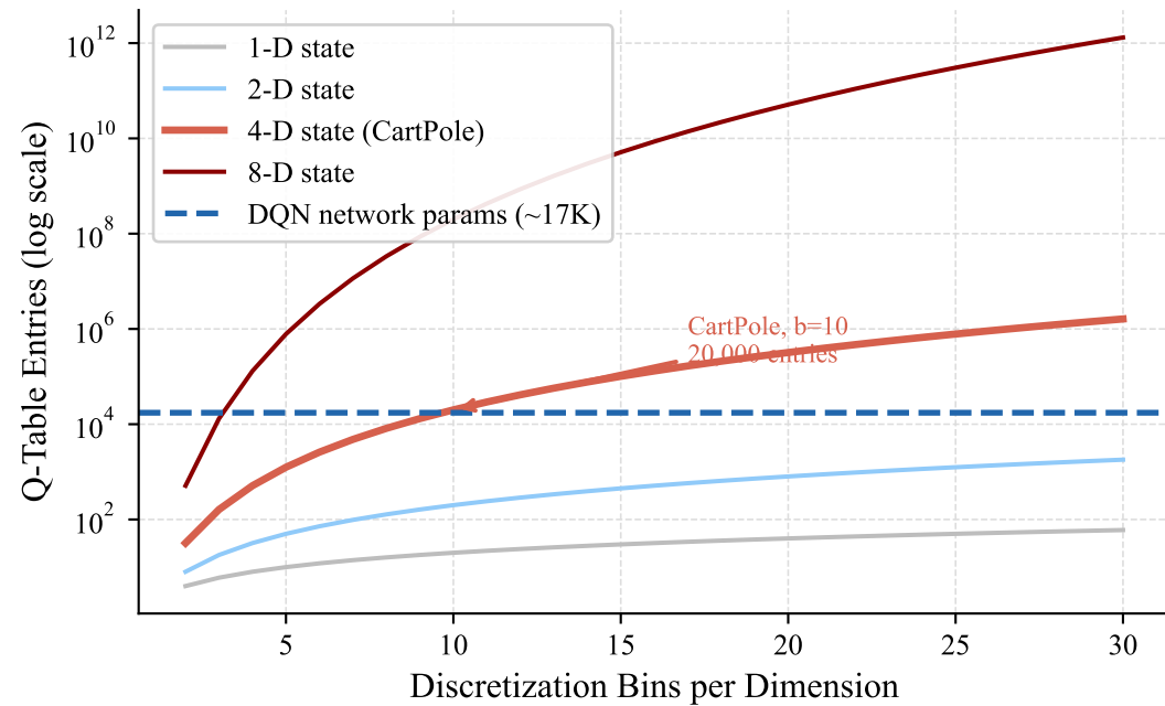
Curse of Dimensionality: Q-Table Size Explosion
