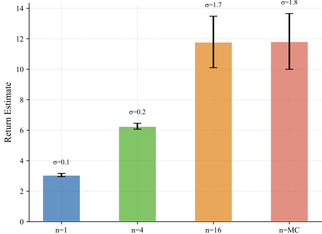
Mean \pm Std of G_0^{(n)} Across 400 Rollouts (error bar = \pm 1\sigma )
