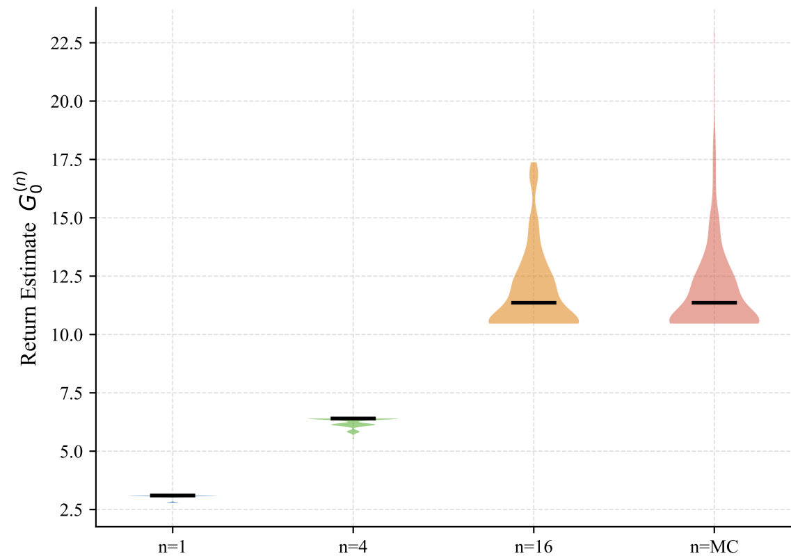
Distribution of n-Step Return Estimates (400 rollouts, same start state, \epsilon=0.25 )
