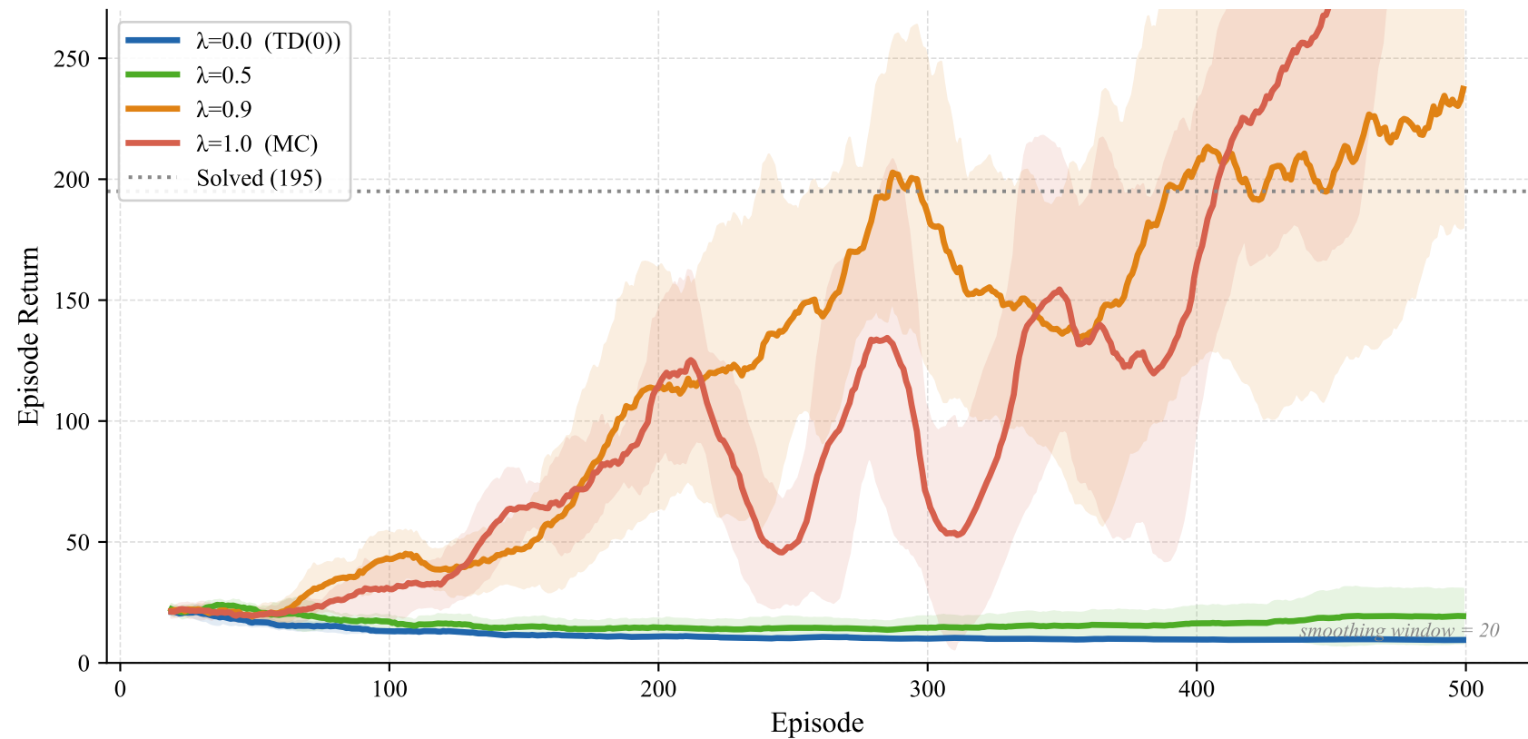
TD( \lambda ) — Effect of \lambda on Learning CartPole-v1 (shading = \pm 1\sigma , 5 seeds)
