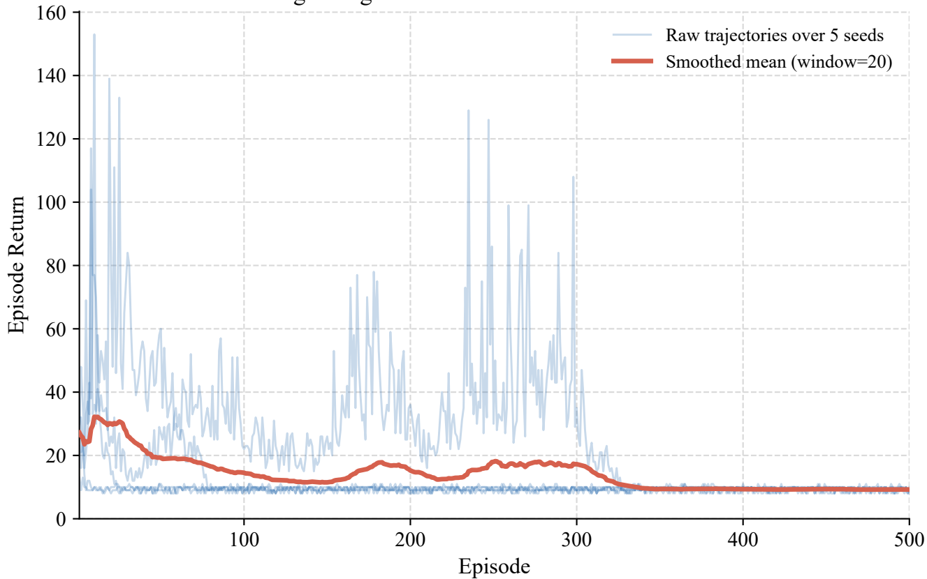
Fig 1. High Variance of Vanilla REINFORCE
