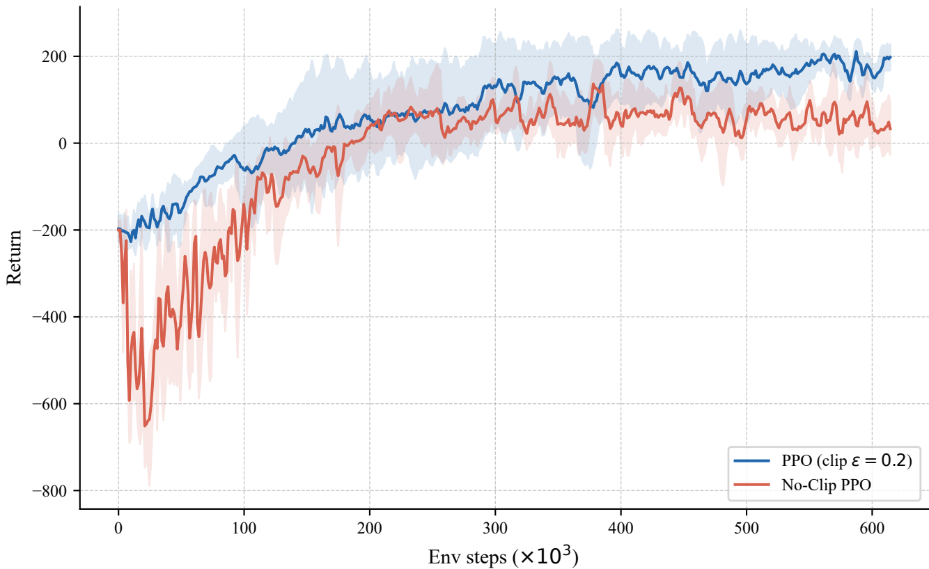
PPO vs No-Clip PPO on LunarLander-v3 (5 seeds, mean \pm std)
