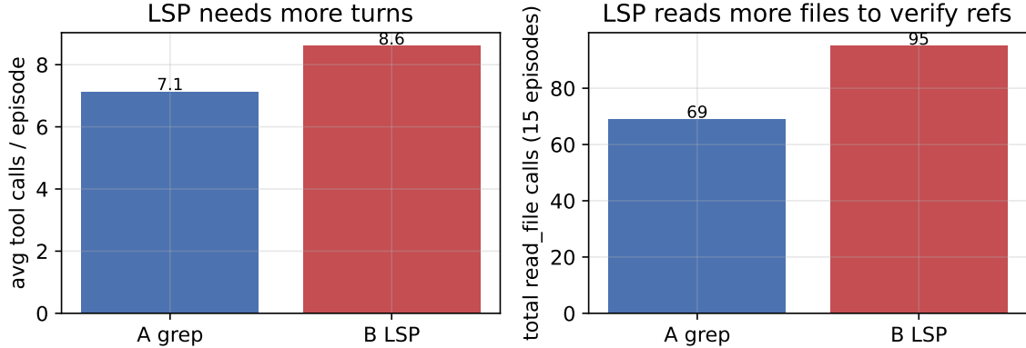
Figure 4: Why the LSP costs +19% tokens on reference tasks. Per-tool-call token cost is nearly identical between arms (163 vs. 160); the difference is call/turn count . Left : the LSP arm issues more tool calls per episode. Right : it issues far more read_file calls. find_references returns locations only ( path:line ), so the agent must open those files to verify each call site; grep returns the matching line’s content inline , often needing no follow-up read. Each extra turn re-bills the accumulated conversation context — so the cost compounds. An LSP tool that returned the referenced line inline would likely erase the penalty while keeping precision = 1.00 (an actionable H-interface fix).
