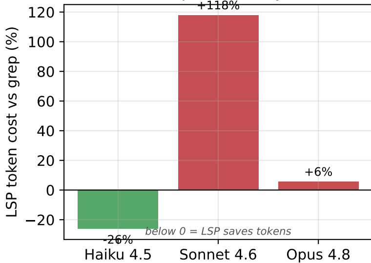
LSP token premium by model
