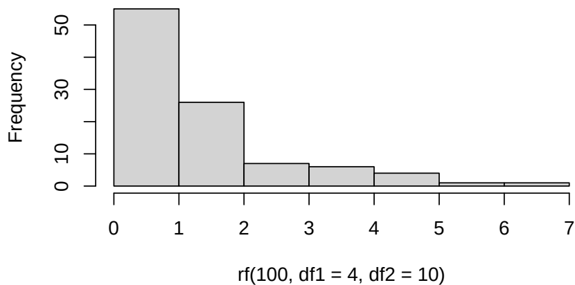
Histogram of rf(100, df1 = 4, df2 = 10)
