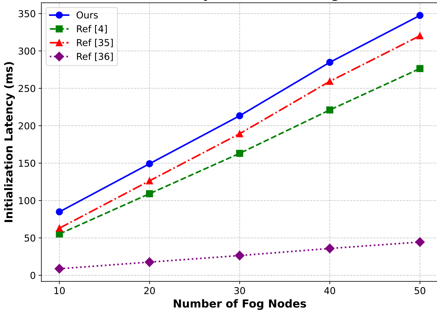
Phase 1: Latency vs Number of Fog Nodes
