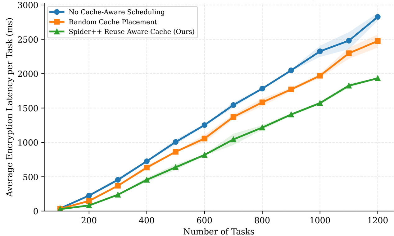
Graph 2: Cache / Reuse-Aware Scheduling
