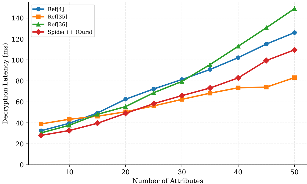
Graph 4: CP-ABE Decryption Cost (User)
