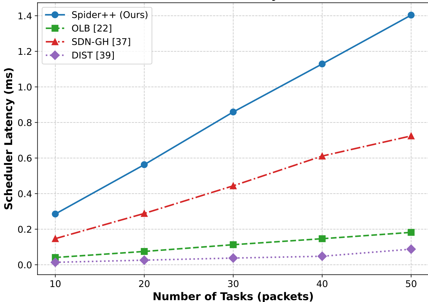
Phase 4: Scheduler Latency vs Task Count
