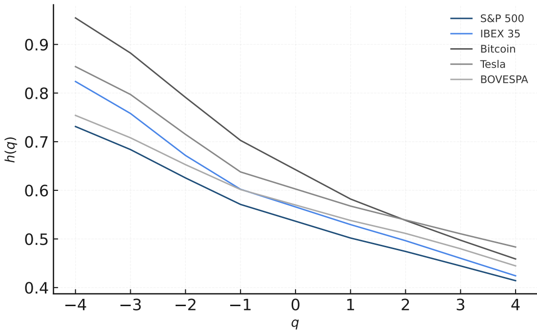
MF-DFA scaling spectra for returns
