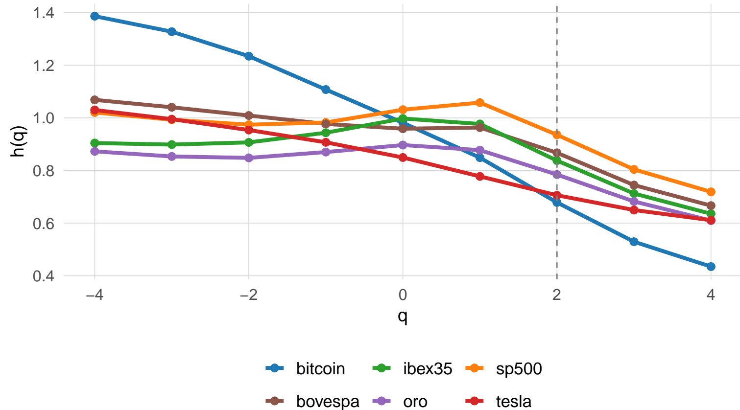
MF-DFA scaling spectra for squared returns (volatility)
