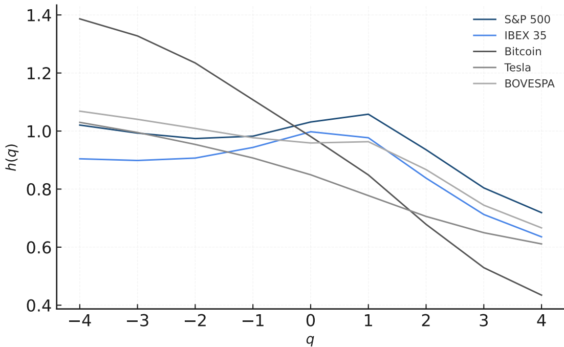
MF-DFA scaling spectra for squared returns (volatility)
