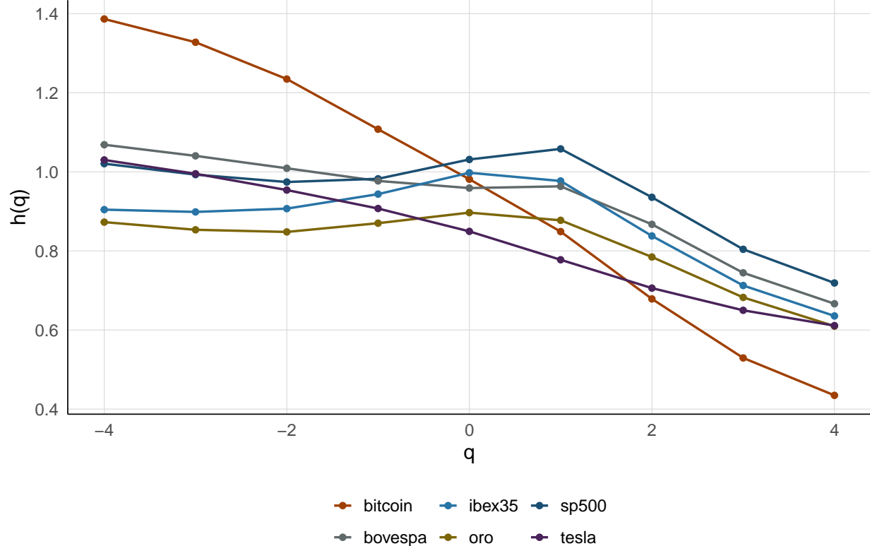
MF-DFA scaling spectra for squared returns (variance)
