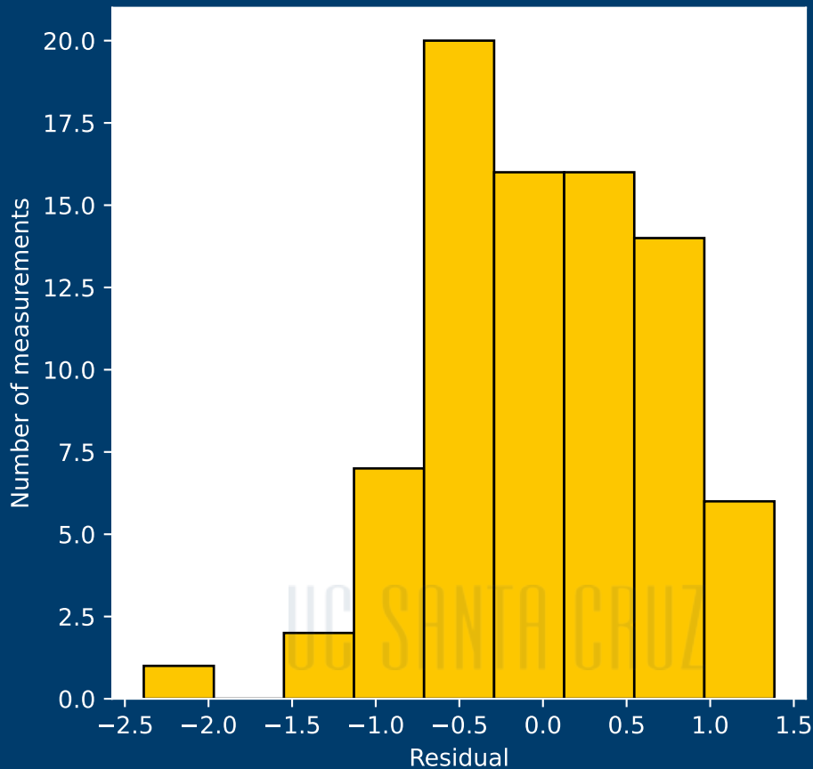
Histogram of Tide Residuals
