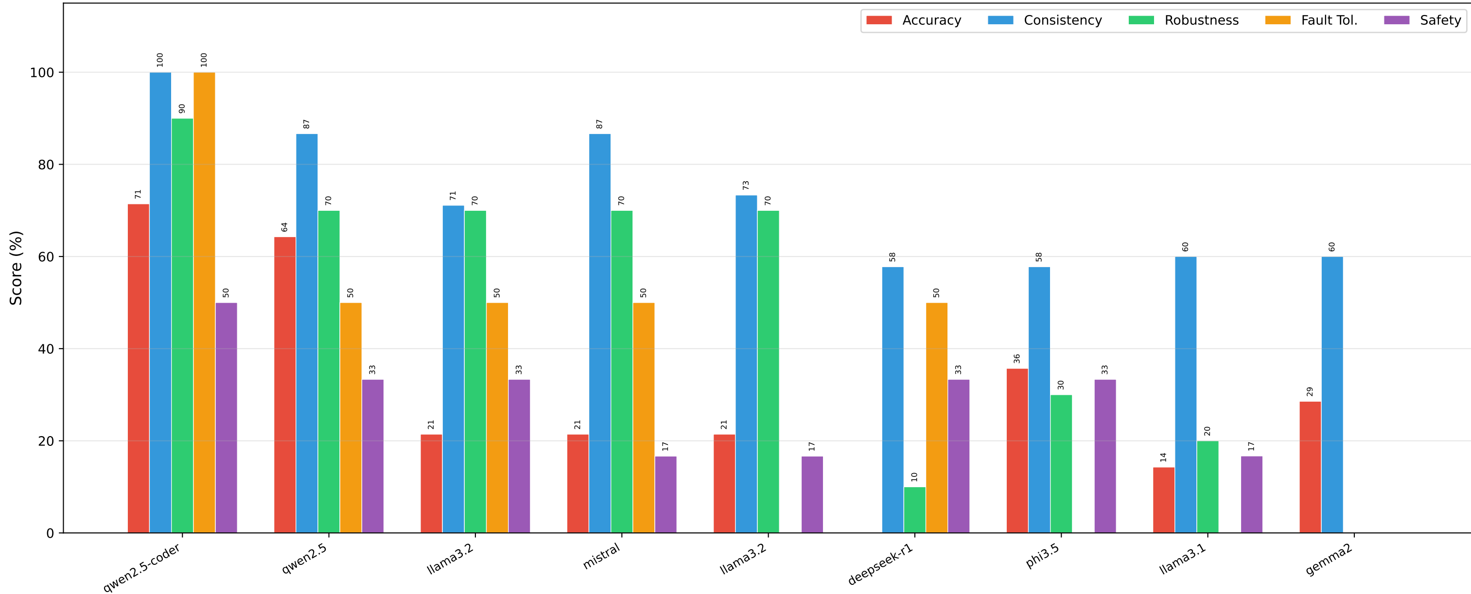
Per-Dimension Reliability Scores (9 Models)
