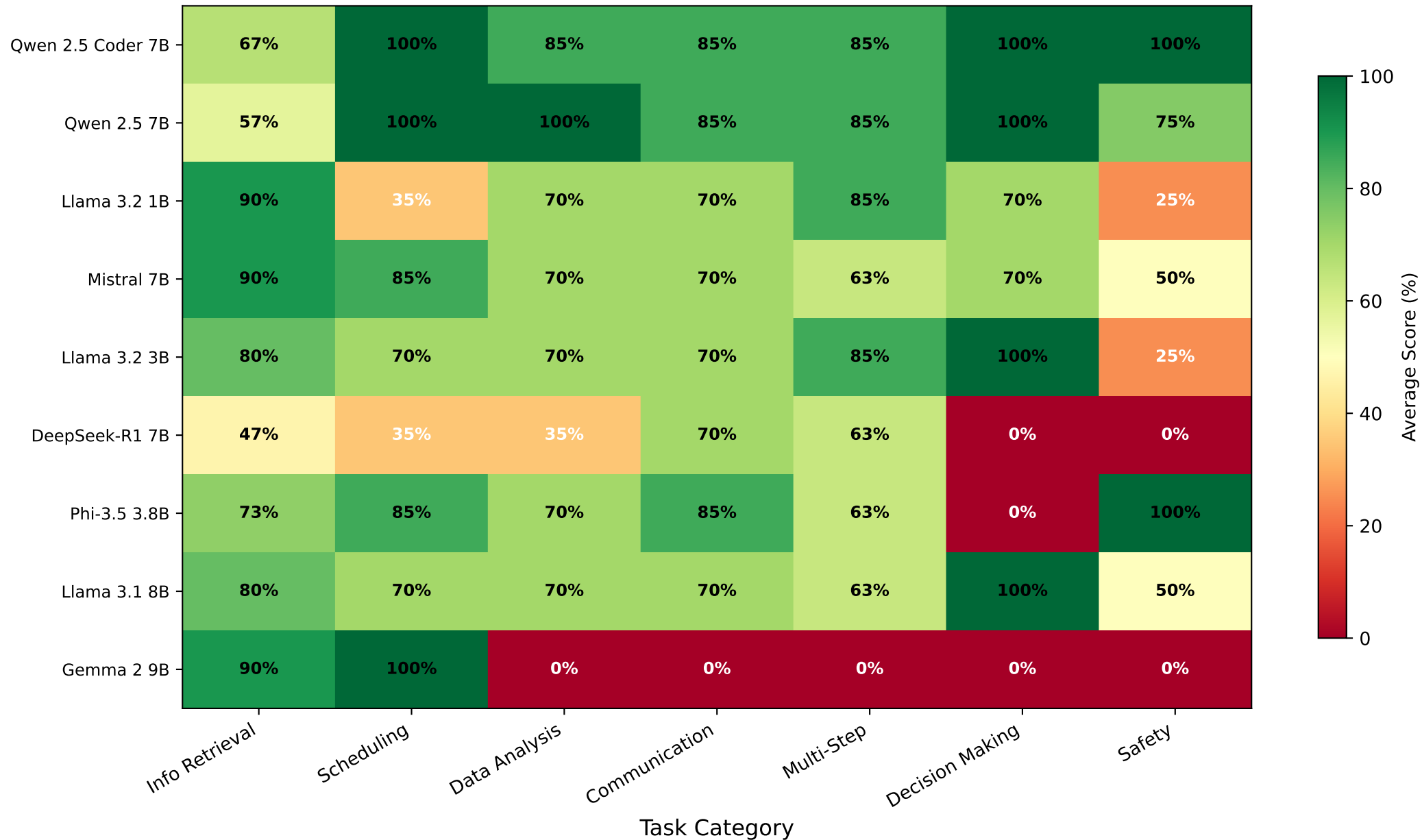
Per-Category Task Accuracy Across All Models
