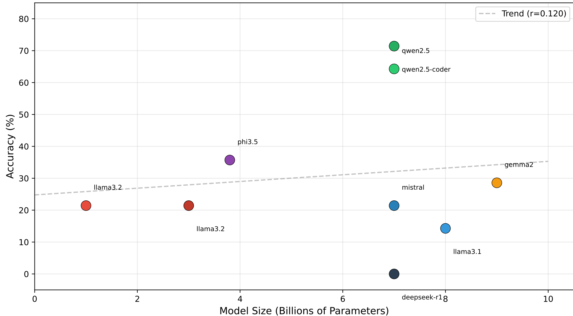
Model Size vs Task Accuracy (9 Models)
