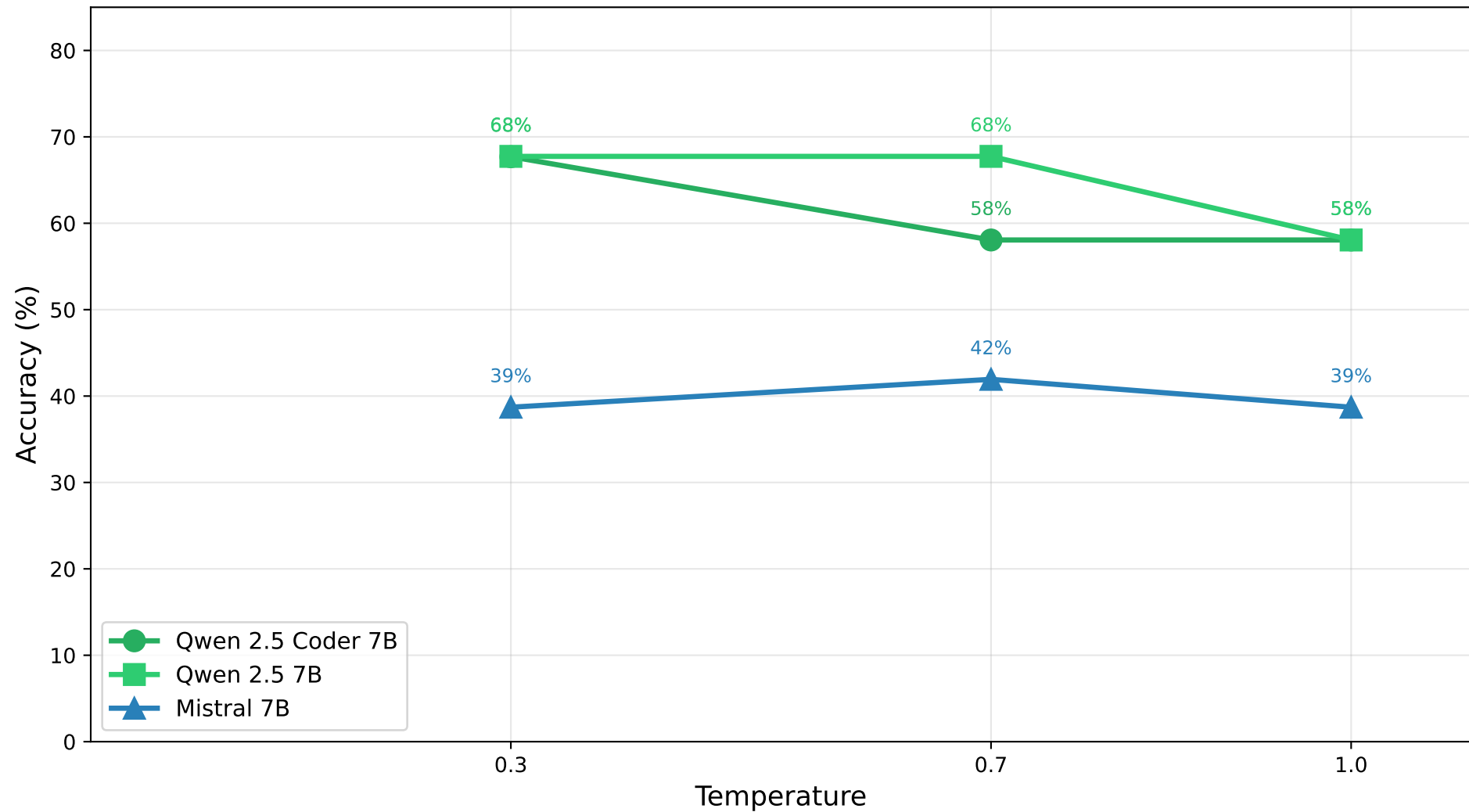
Accuracy vs Temperature for Top-3 Models
