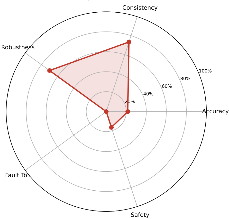
llama3.1 8b (8.0B) Composite: 24.2%
