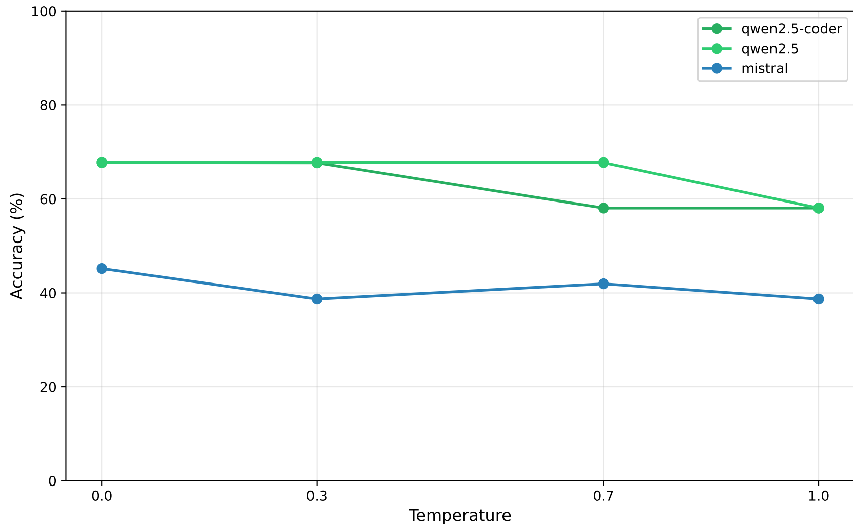
Accuracy vs Temperature (31-Task Suite)
