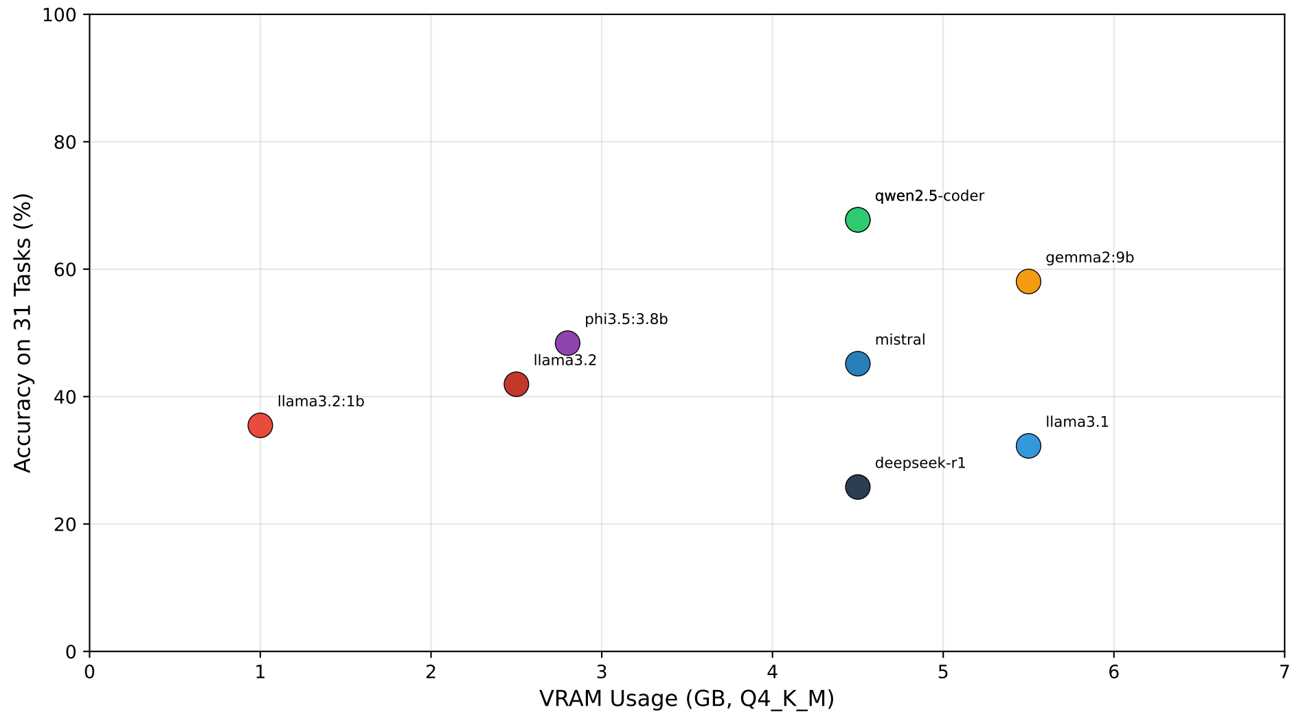
Cost (VRAM) vs Reliability (31-Task Accuracy)
