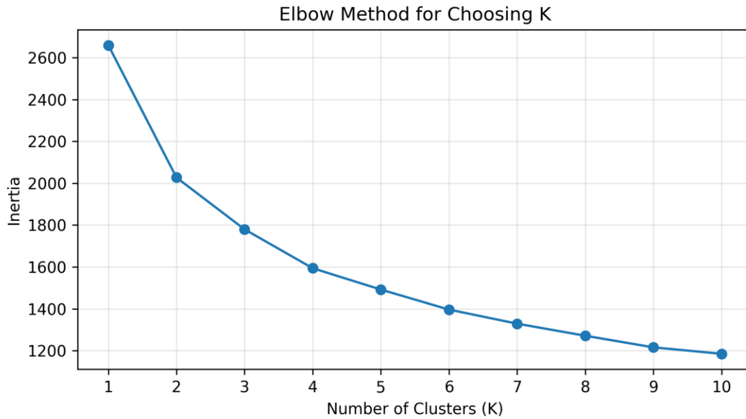
Figure 4: Elbow Method for choosing K
