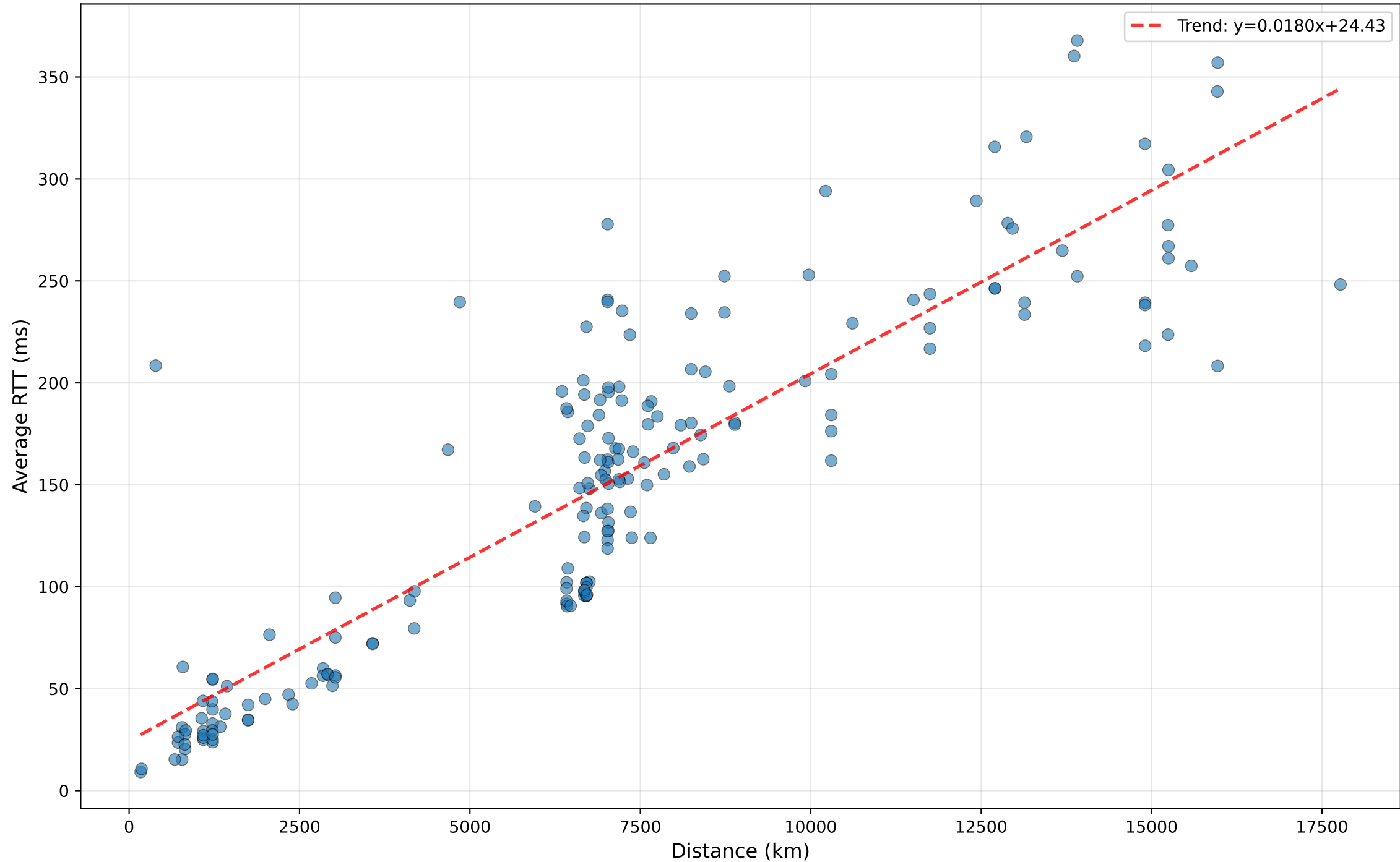
Network Latency vs Geographic Distance From: West Lafayette, United States
