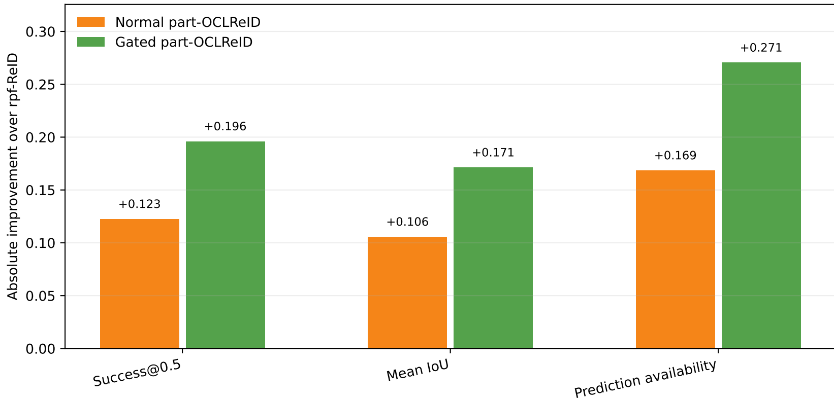
Improvement over rpf-ReID on the AGHRI test set
