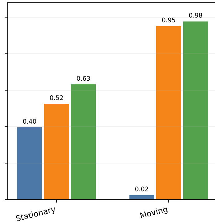
Prediction availability
