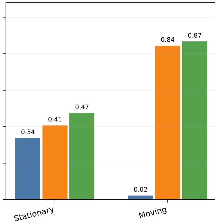
Mean IoU
