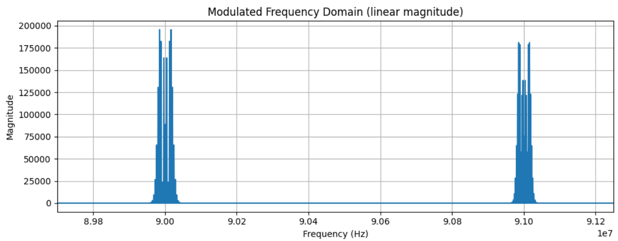
Frequency Domain Plot
