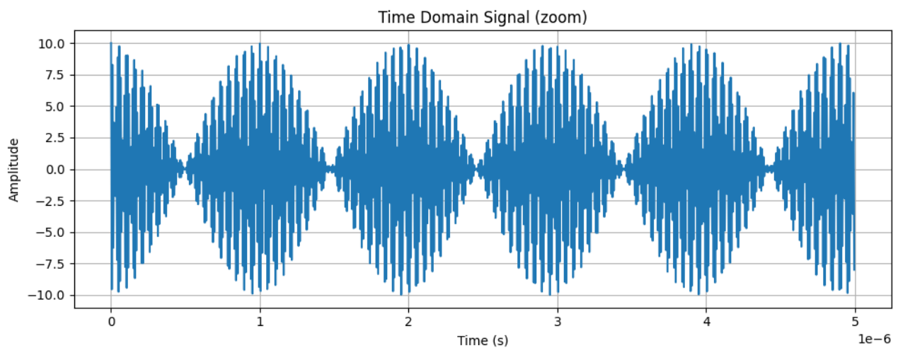
Signal in Time Domain (Task 1)
