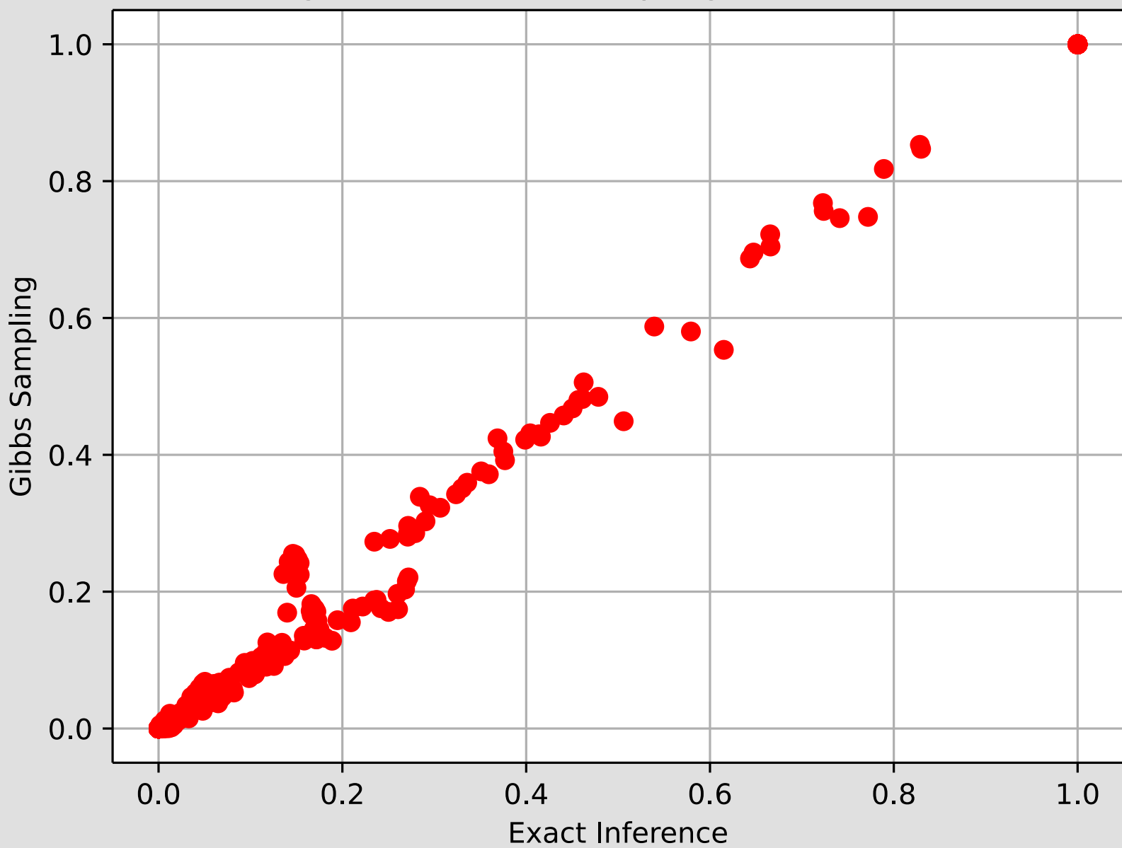
Convergence of Gibbs Sampling vs. Exact Inference
