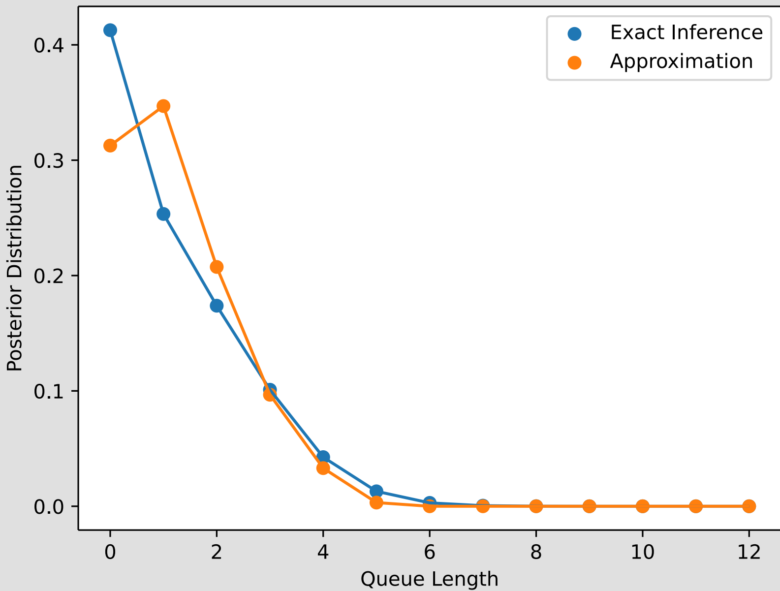
Exact vs. Approximation JSD: 0.105
