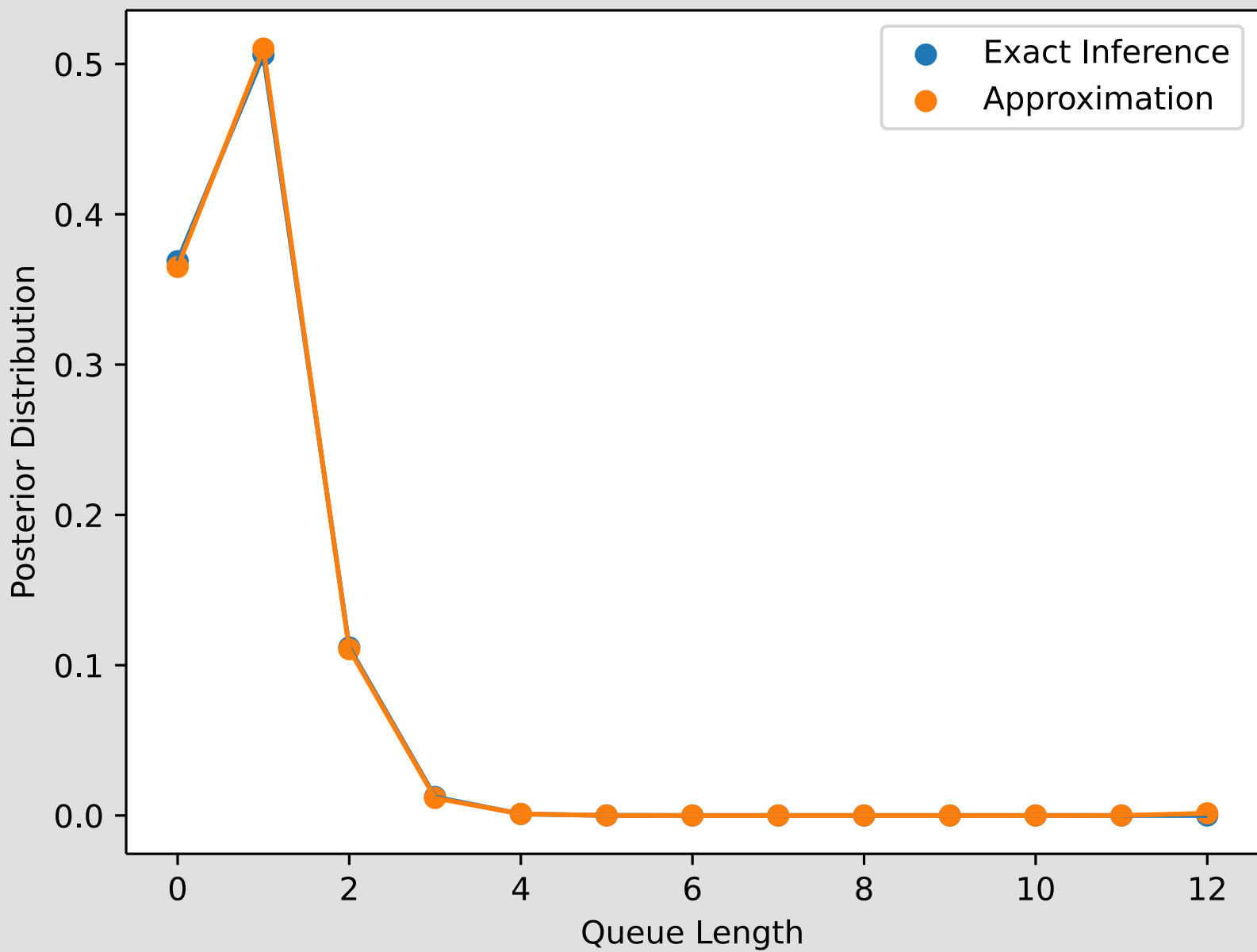
Exact vs. Approximation JSD: 0.023
