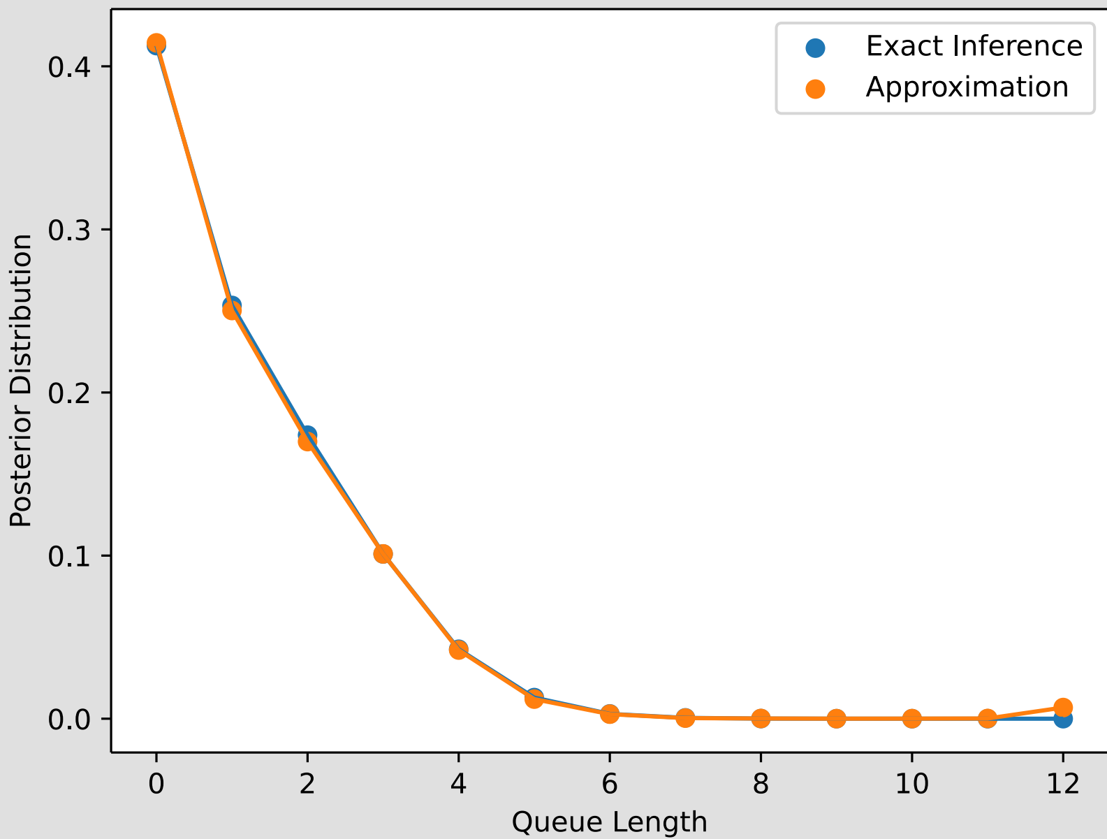
Exact vs. Approximation JSD: 0.05
