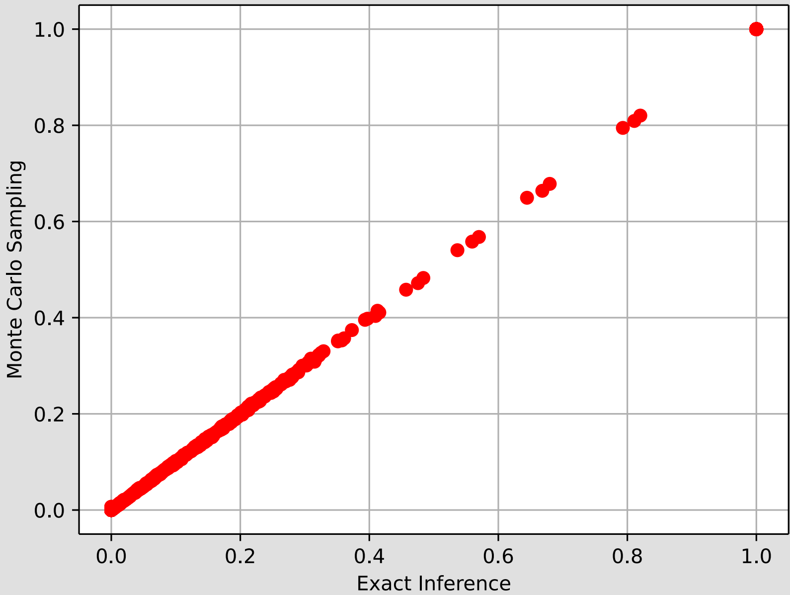
Convergence of Monte Carlo Sampling vs. Exact Inference
