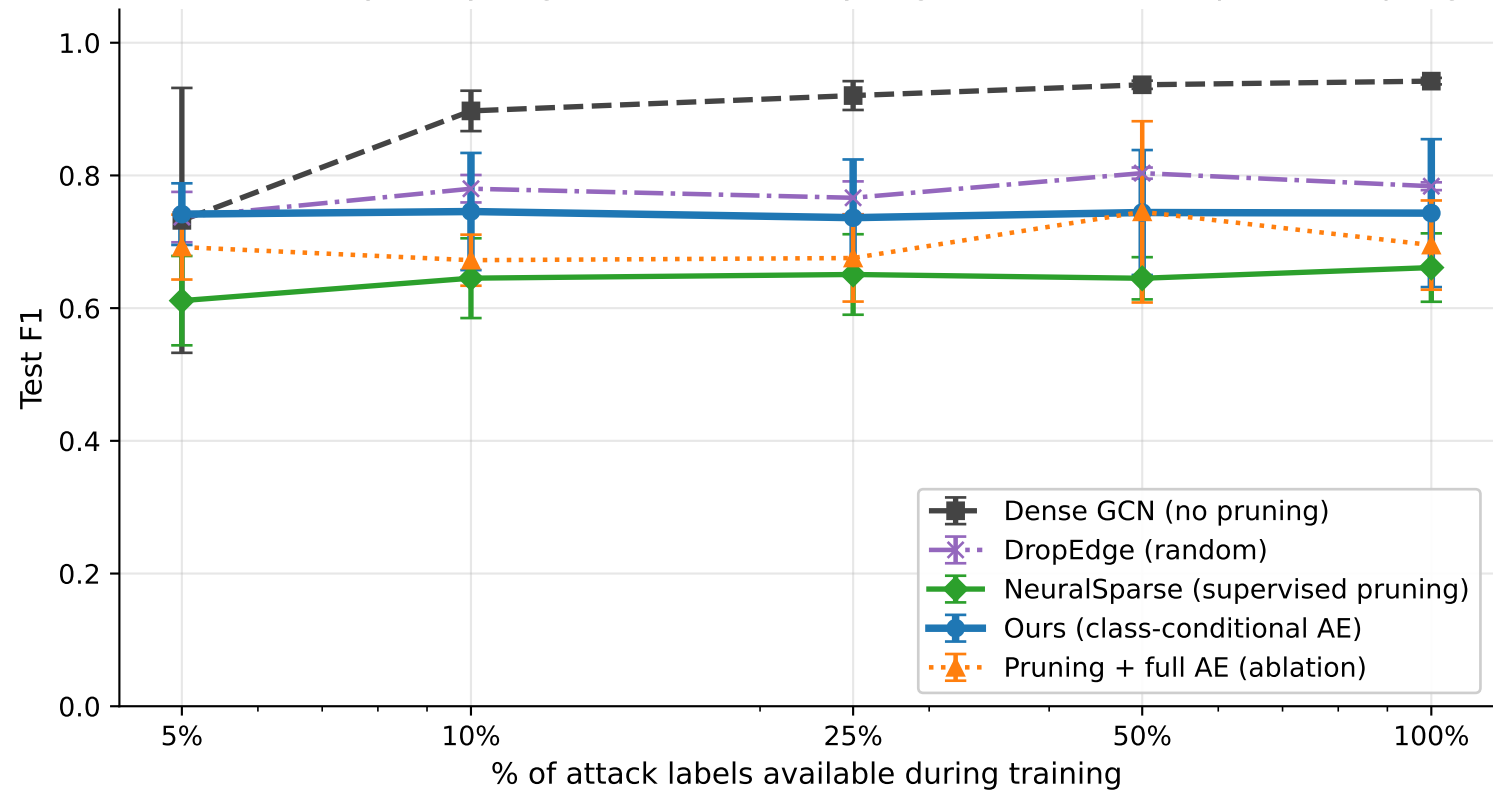
Label-Efficiency Study (high-noise: 60% noisy edges) — vs. NeuralSparse, DropEdge
