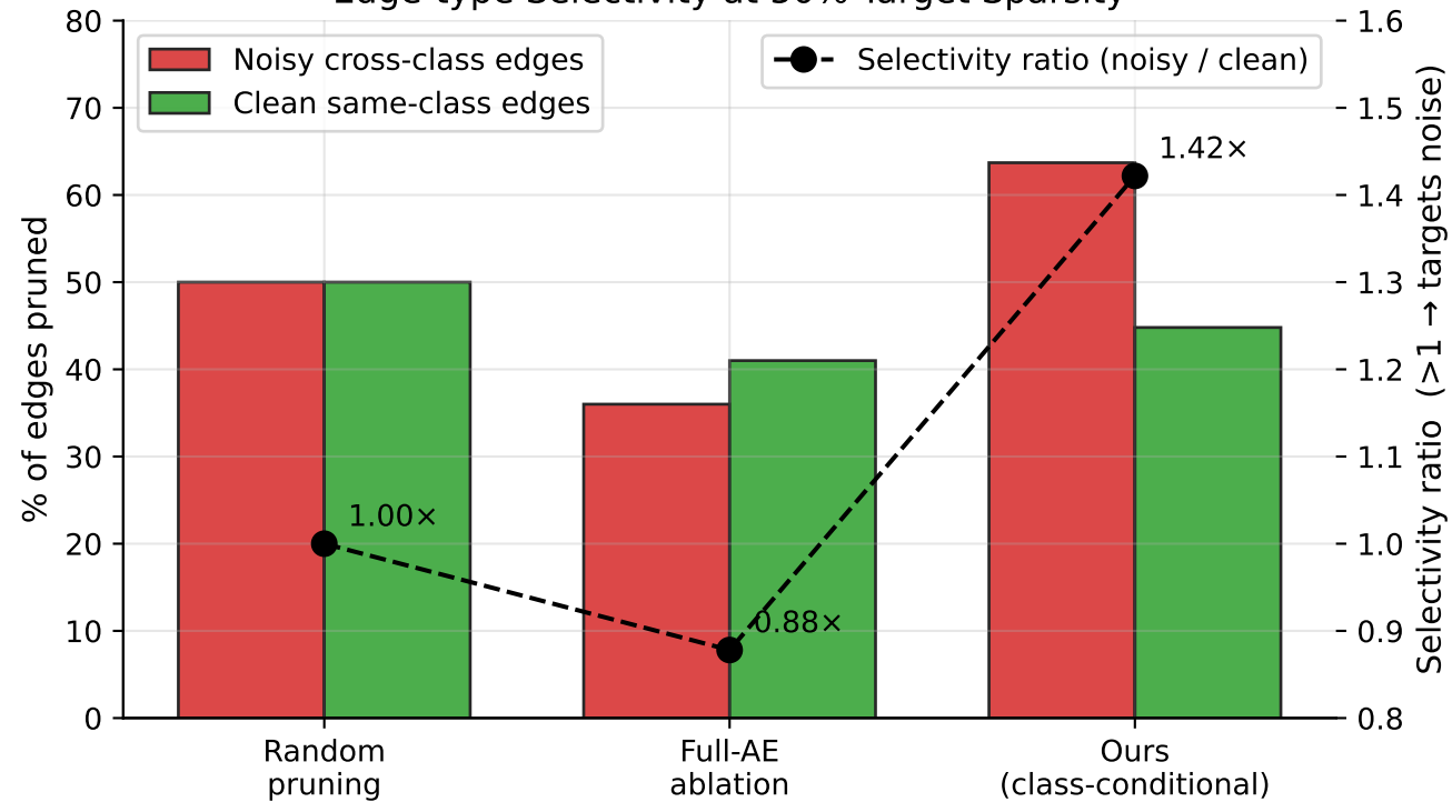
Edge-type Selectivity at 50% Target Sparsity
