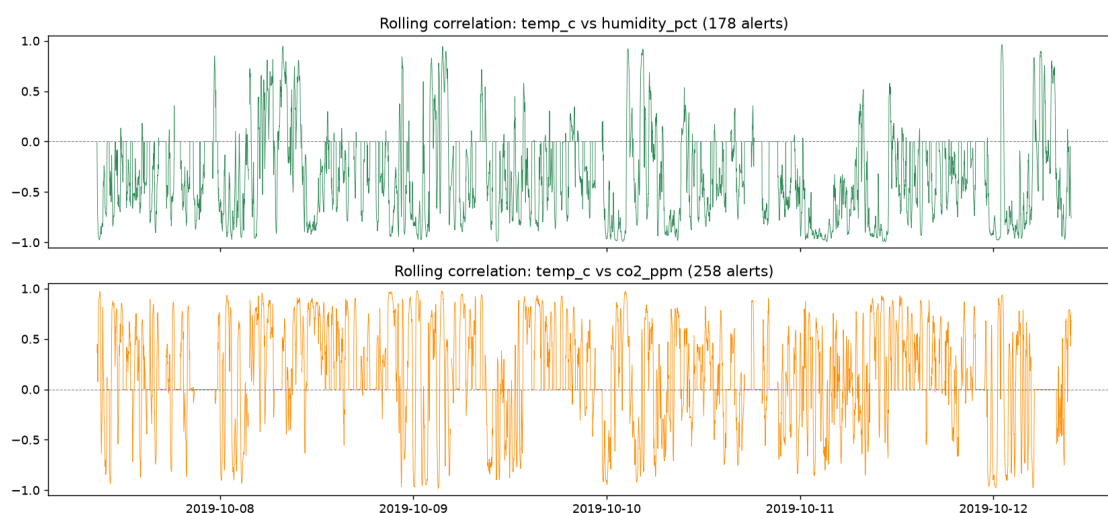
Figure 4: Rolling correlation for both pairs. The co2 pairing (bottom) oscillates far more erratically than the humidity pairing (top), consistent with variance-floor instability rather than a real relationship.
