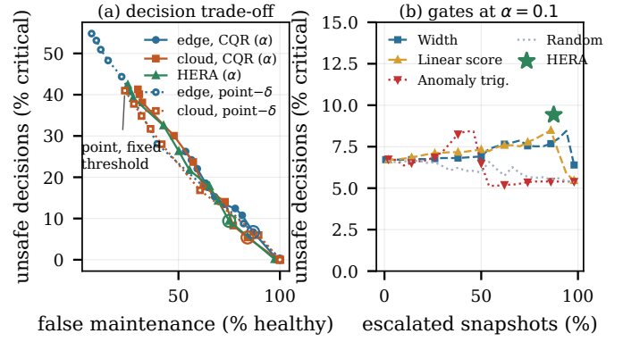
Fig. 3. (a) Unsafe decisions vs. false maintenance when sweeping \alpha (calibrated) or margin \delta (point); circles mark \alpha = 0.1 . (b) Unsafe decisions vs. escalation budget for gates operating on the same \alpha = 0.1 edge intervals.
