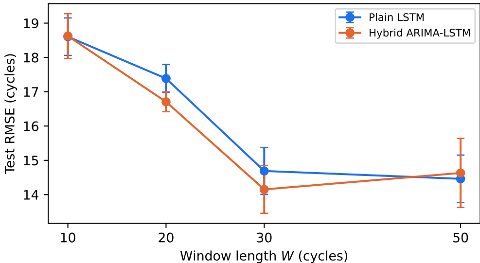
FD001: window length vs. RMSE, mean \pm std over 6 seeds
