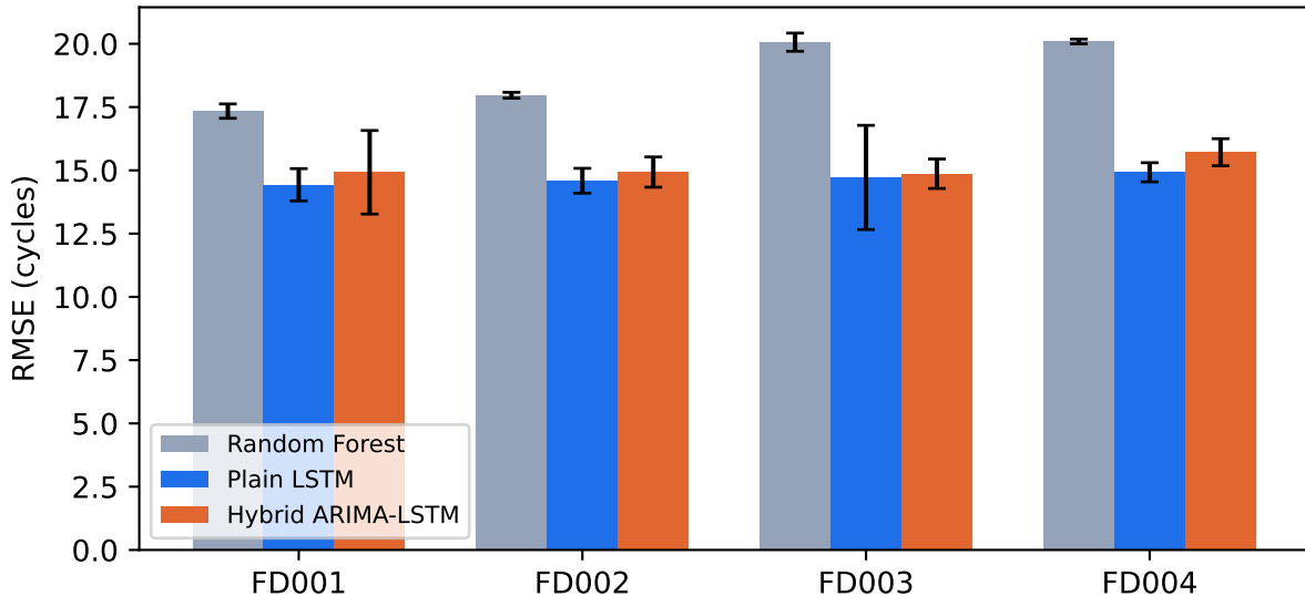
RUL prediction RMSE, mean \pm std over 6 seeds
